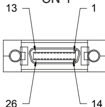
MDR 26 Position Receptacle Camera End CN-1
