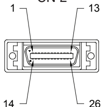
MDR 26 Position Plug Frame Grabber End CN-2
