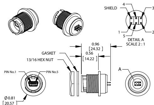
DCP-USBNB-MNHD USB Mini-B to PC Tails
