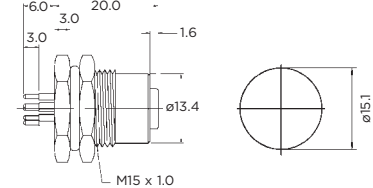
Female PCB Pins Hexagonal Front Nut
