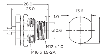
Male PCB Pins Hexagonal Front Nut
