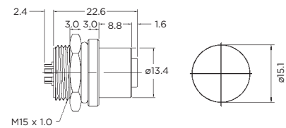
Female PCB Pins Hexagonal Front Nut
