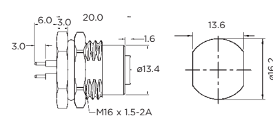
Female PCB Pins Hexagonal Front Nut
